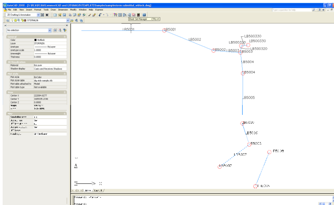
Figure 2 AutoCAD 2008 window showing Sample_storm.dwg sewer lines.
