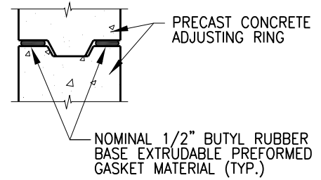
GASKET DETAIL
