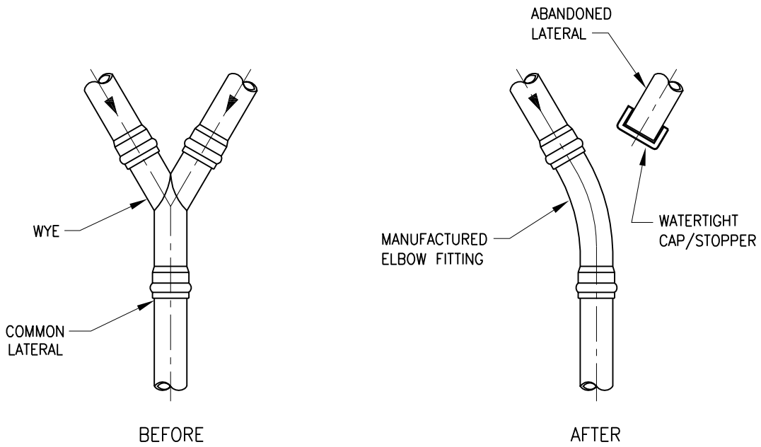
SHARED LATERAL CAP LOCATION PLAN VIEW DETAIL
